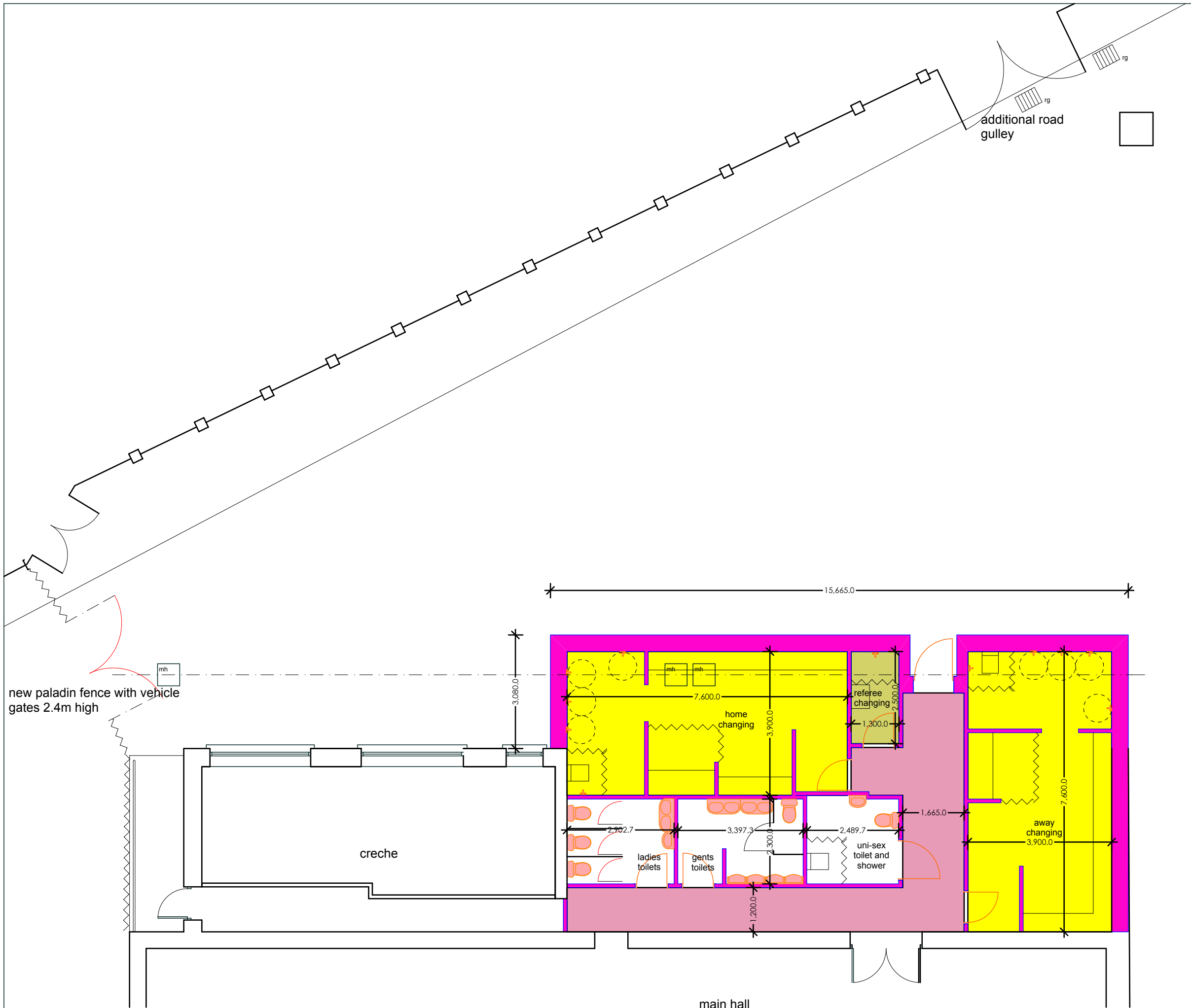
Proposed Plan - Toilets & Changing Rooms 110m2
